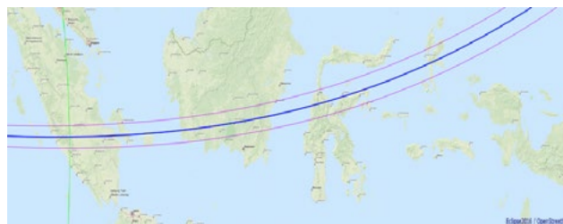
Gambar Jalur lintasan Gerhana Matahari Total 2016
